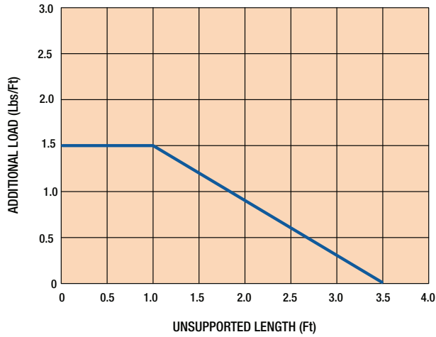
P-SERIES LOAD CHART
